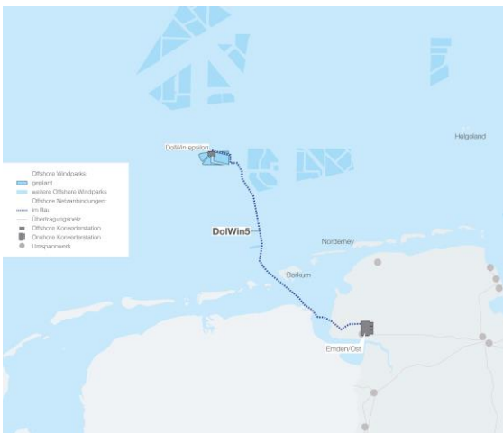
Image caption: Schematic illustration of offshore grid connection project DolWin5
